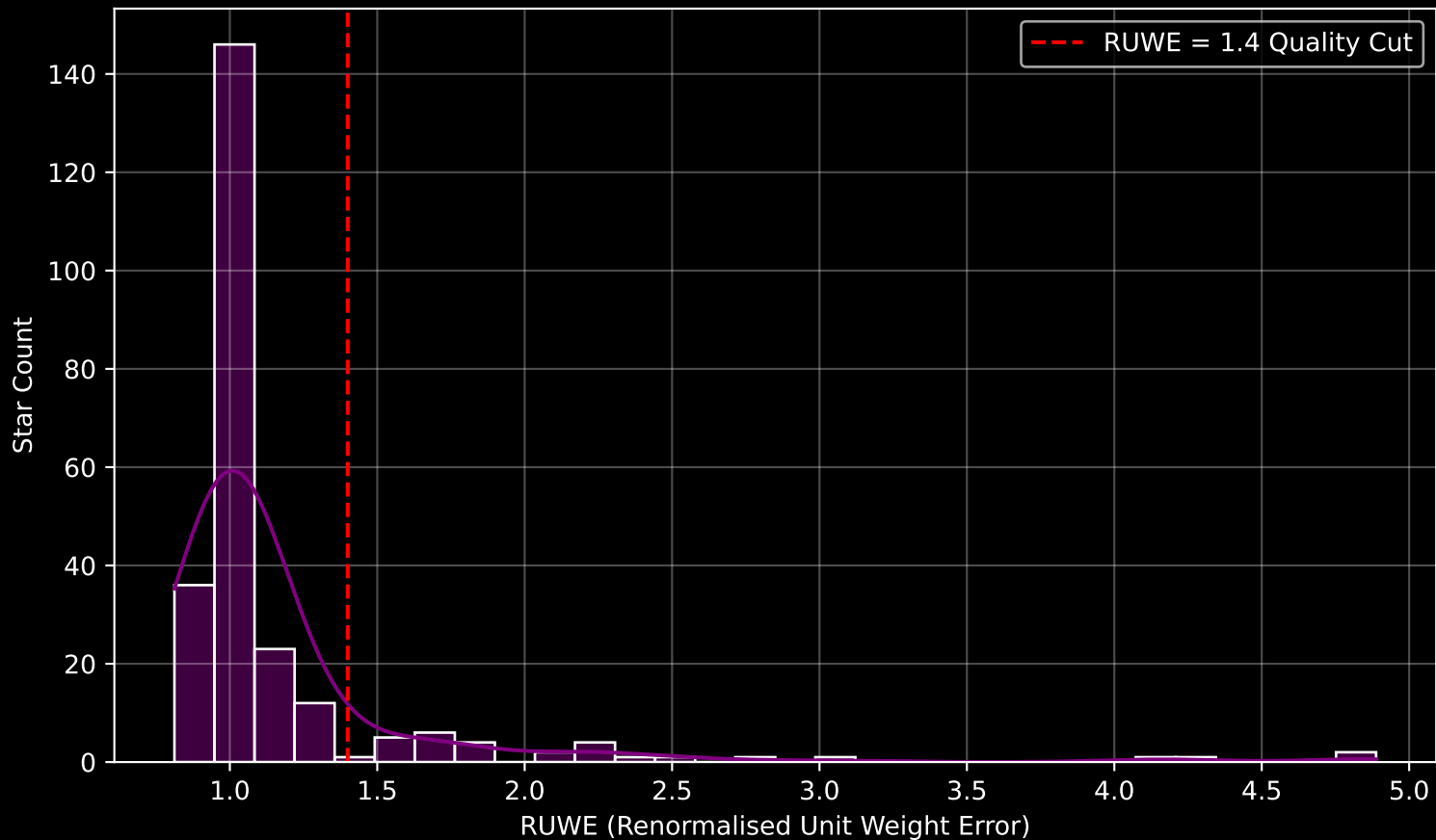
GALAH DR4 Field [2884] RUWE Distribution (n= 247)
