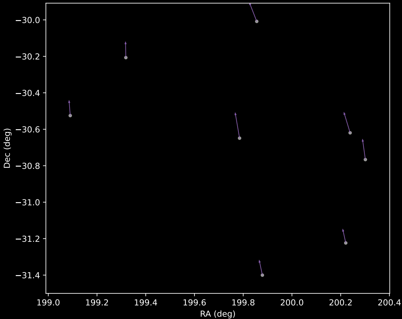
GALAH DR4 Cluster 8 Proper Motion Vectors (n=8)
