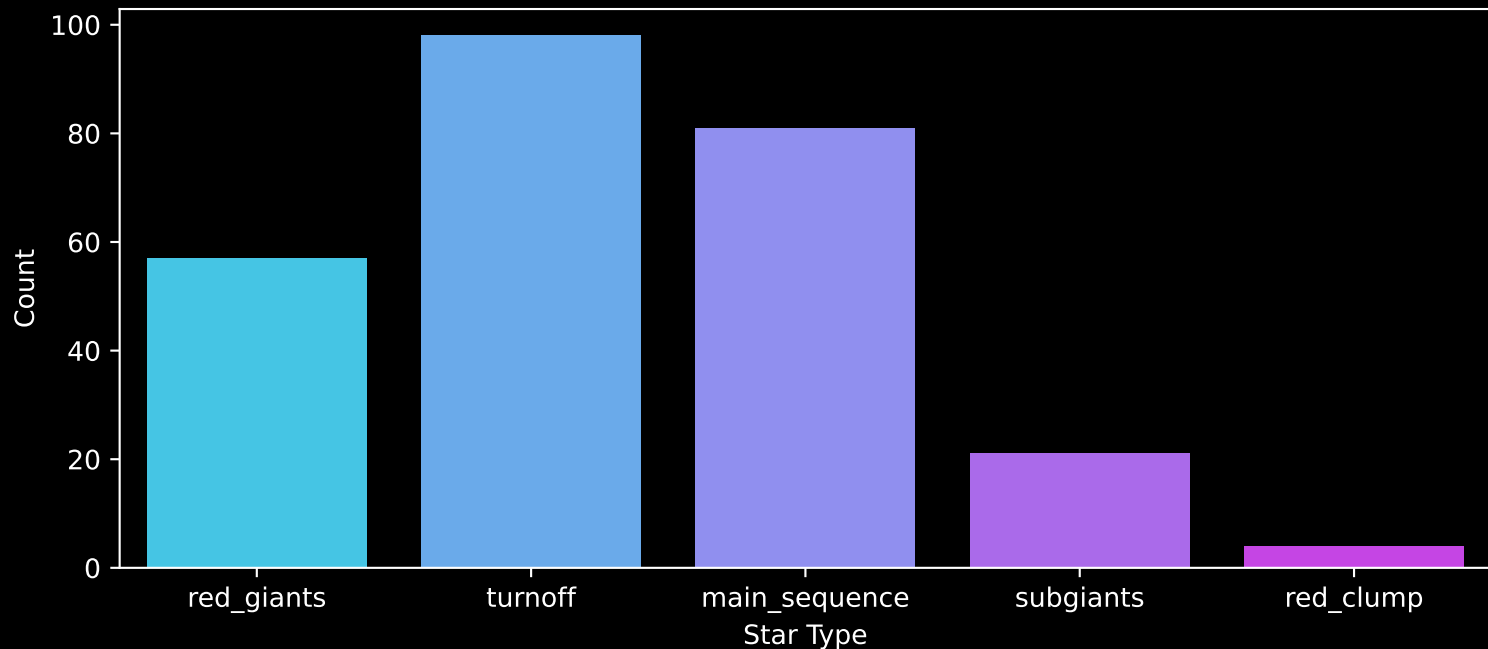
GALAH DR4 Field: [2884] Count plot of Star Type
