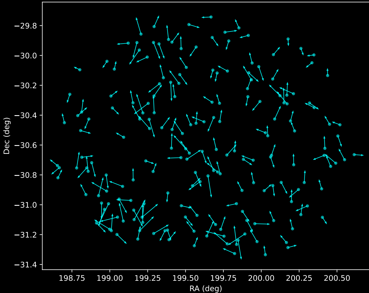
GALAH DR4 Noise Stream Proper Motion Vectors (n=190)
